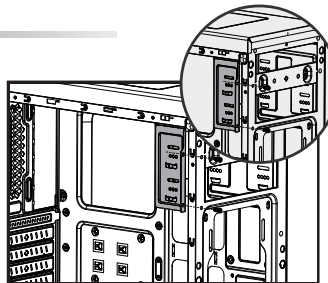
Install ODD tray.
